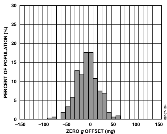
Figure 7. X-Axis Zero g Offset at 25°C, V_s = 1.8\text{ V}
